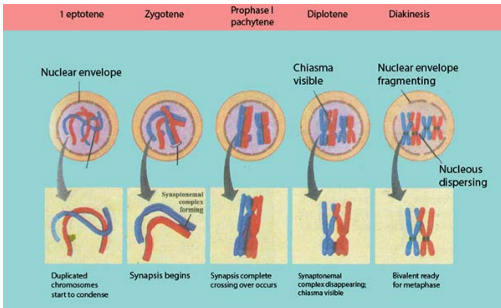
Fig. 21.5 Chiasmata formation
